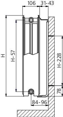
type 22
