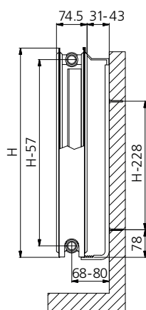
type 21s
