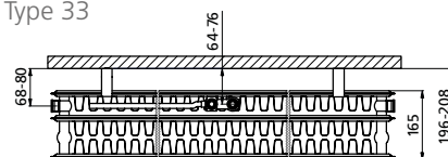
Montage links
