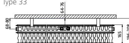
Montage links
