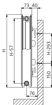
type 21s
