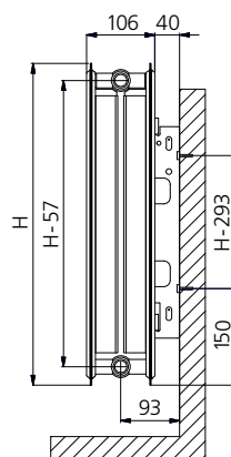
type 22
