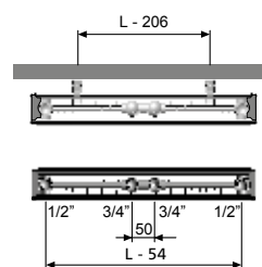
type 22
