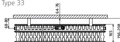
Montage links
